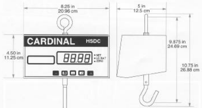
Overall height of HSDC with produce pan is 34.75"
